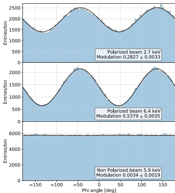
Fig. 18. Example of modulation curves for 2.7 keV and 6.4 keV, \sim 100\% polarized and 5.9 keV un-polarized X-rays. We note that the underlying selection cuts used are not necessarily identical to those that will be used for the analysis of flight data, and, as a consequence, the final modulation figures might be slightly different.
