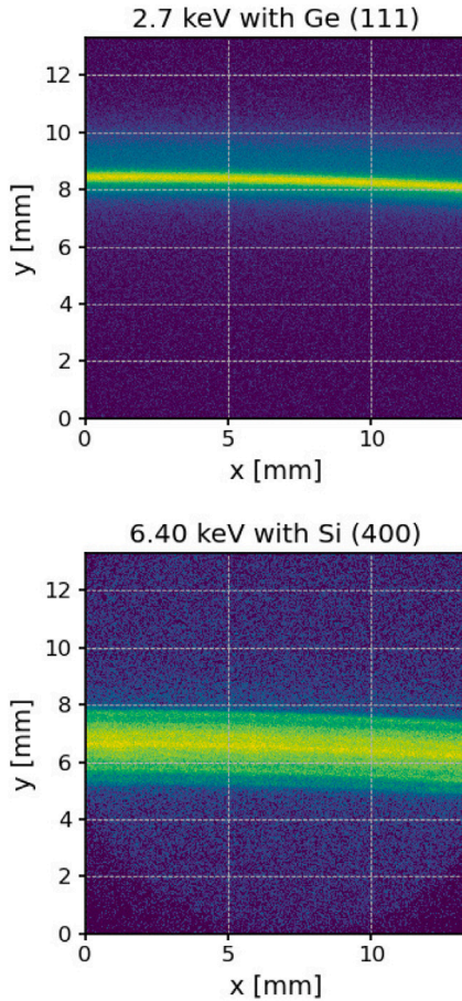
Fig. 18. Image with the ICE test imager of the photons generated with the polarized source without collimators. In this condition, diffracted X-rays forms a “Bragg” arc on the detector, whose width depends on both the source and the crystal used. On the top there is the Bragg arc obtained with the X-ray tube with Rh anode and the Ge (111) crystal; on the bottom there is the Fe X-ray tube with Si (400) crystal.
