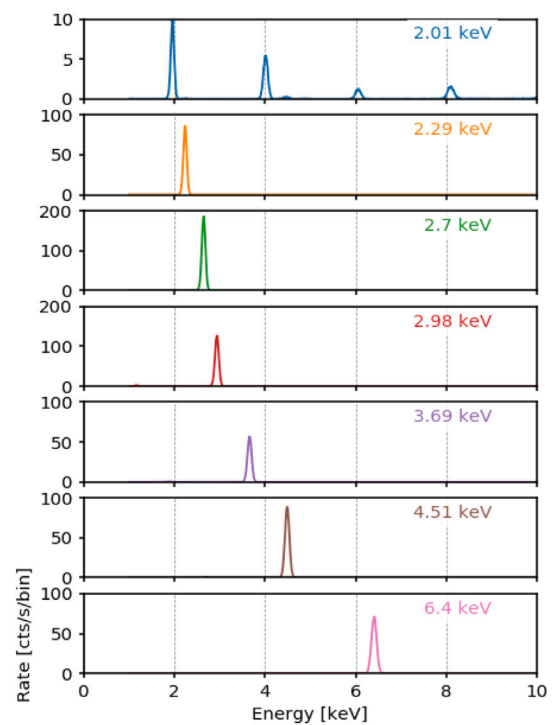
Fig. 16. Spectra from polarized sources measured with the ICE test spectrometer.
