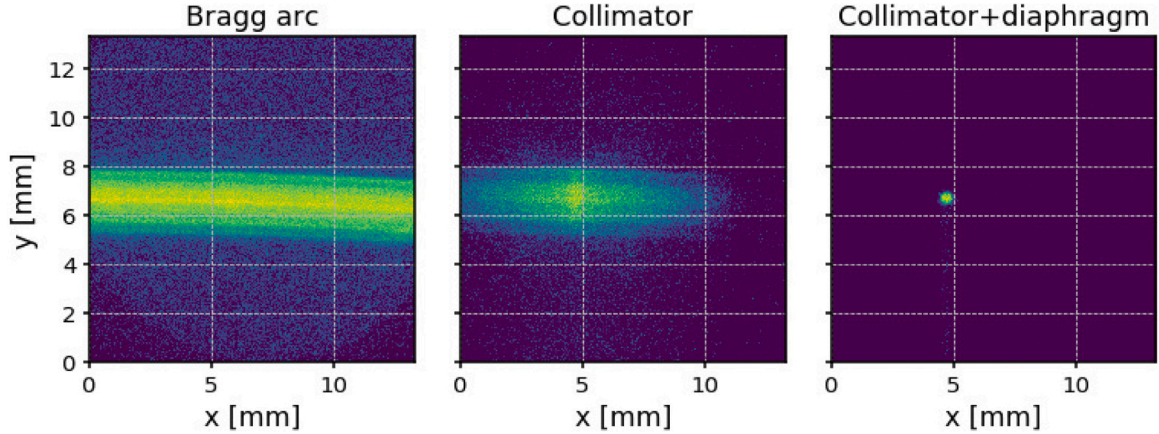
Fig. 20. Basic steps for polarized source alignment. The Bragg arc is visible when no collimator or diaphragm is present. Adding a collimator, only the Bragg arc corresponding to photon passing through the collimator is visible. The final step is to center a diaphragm in the brightest region of the remaining Bragg arc. At the end of the procedure, the beam is measurable as the line passing through the diaphragm and forming with the crystal plane an angle equal to the Bragg one.
