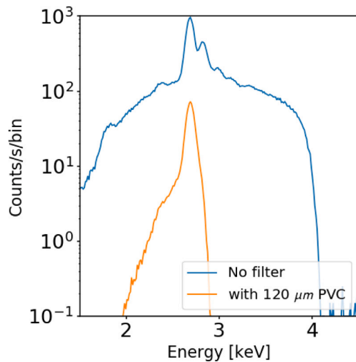
Fig. 8. Example of the effect on the spectrum of direct X-ray tube with Rh anode with and without X-ray filter 120 \mu\text{m} thick to select the L\alpha fluorescence line.
