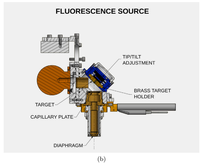
Fig. 9. Drawing of the direct unpolarized source (a) and of the fluorescence unpolarized source (b).
