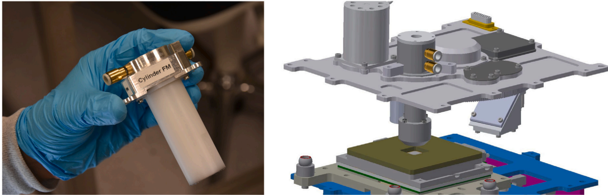
Fig. 25. Cylinder to flow helium in the path from a X-ray source to the detector (left). The figure to the right shows the cylinder mounted inside the DU during calibration.
