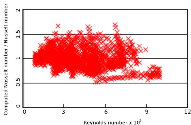
Fig. 8. Ratio of the Nusselt number computed with a typical correlation to the experimental Nusselt number versus Reynolds number (figure taken from Ref. [18]).
